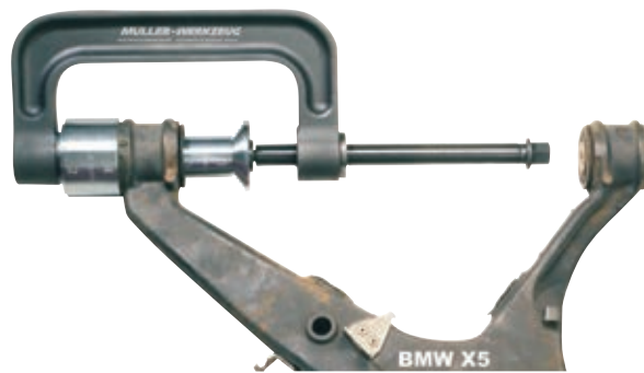
Example of use: C-Frame + press and pull sleeve kit
