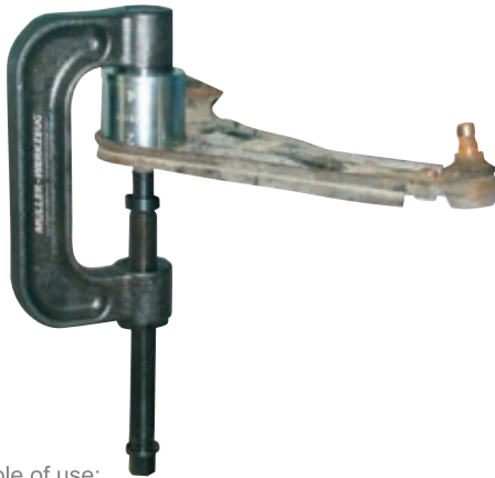
Example of use: C-Clamp type 1 + press and pull sleeve kit
